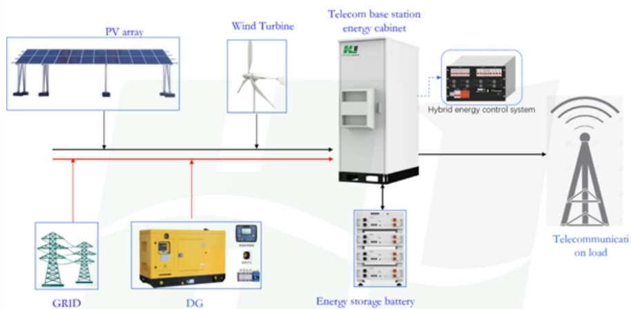
Base station energy composition diagram
