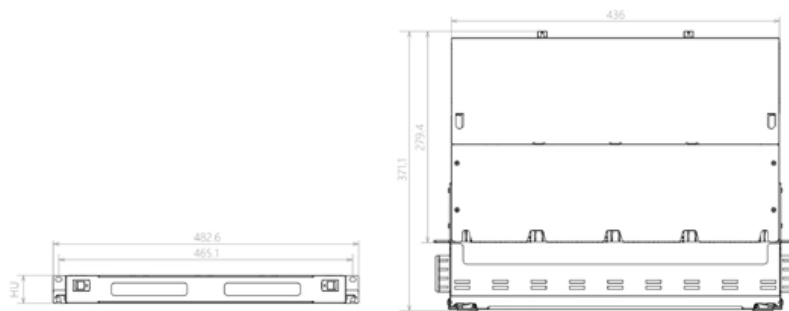
Key dimensions
